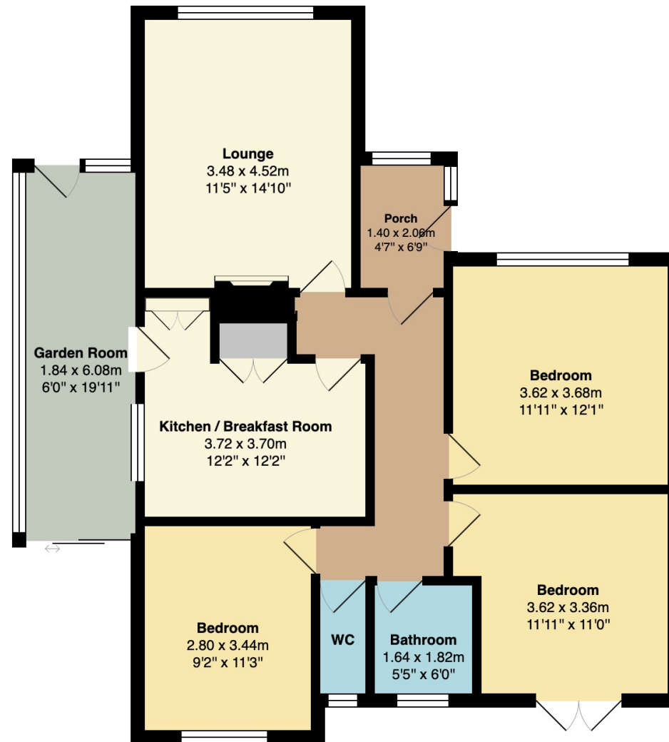
Ground Floor Area: 94.5 m 2 ... 1017 ft 2
